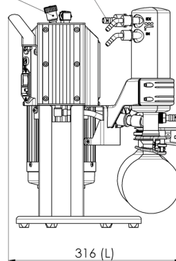
VACUUBRAND MD 1C +AK+EK Version 05
